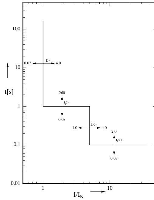
Figure 8.4: Definite time overcurrent relay
