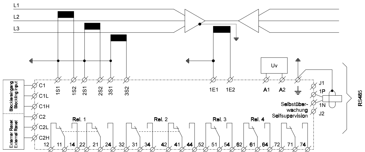
Figure 3.1: Connection diagram XRI1-IE
