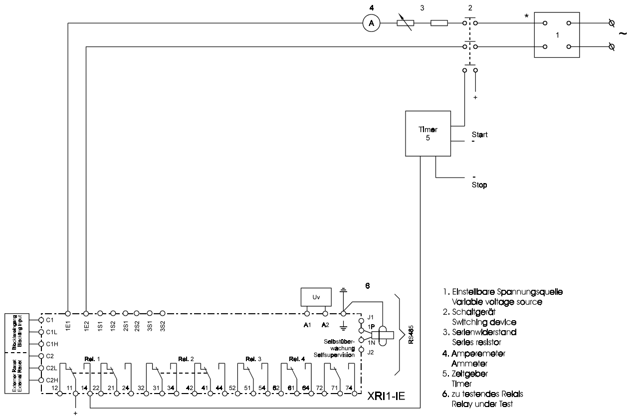
Figure 7.1: Test circuit
