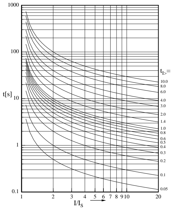
Figure 8.1: Normal Inverse (type A)
