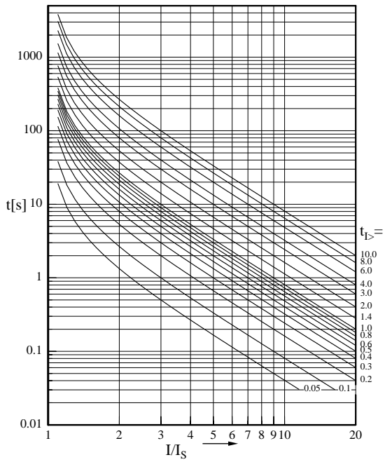
Figure 8.2: Extremely Inverse (type C)
