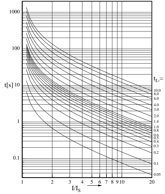
Figure 8.3: Very Inverse (type B)
