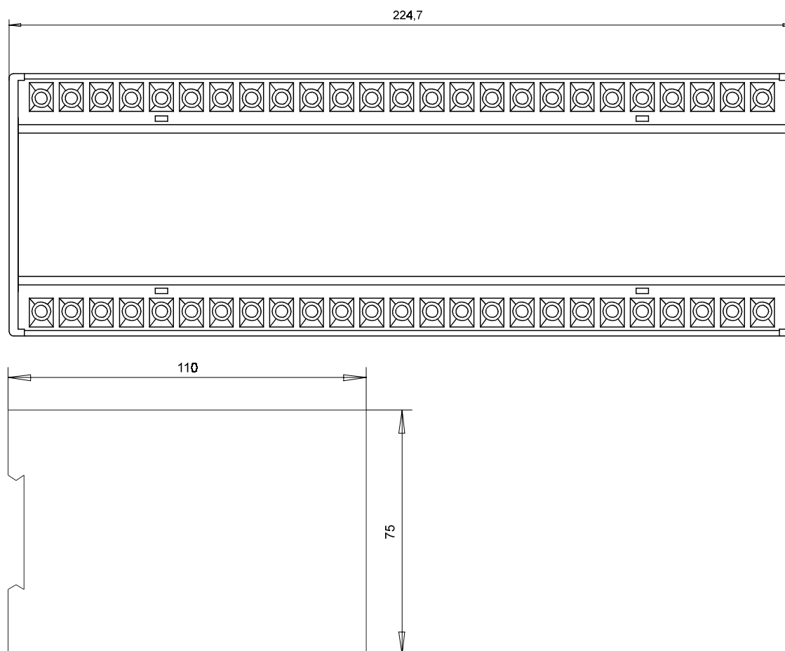
Figure 8.5: Dimensional drawing; dimensions in mm
