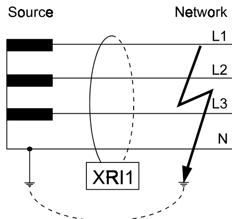
Figure 4.2: System earth fault protection
