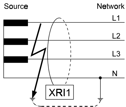
Figure 4.1: Generator stator earth fault protection
