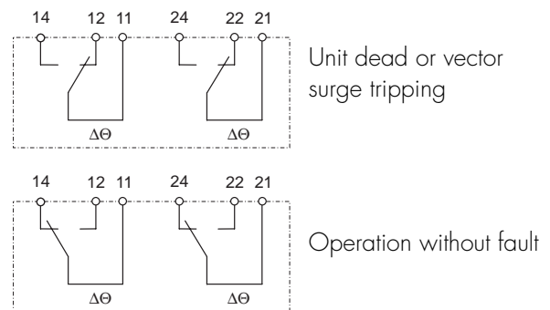
Fig. 2.4: Contact positions of the output relays
