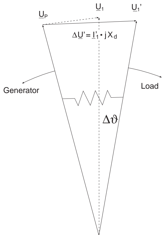
Fig. 3.4: Voltage vectors at mains failure
