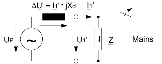
Fig. 3.3 Equivalent circuit at mains failure
