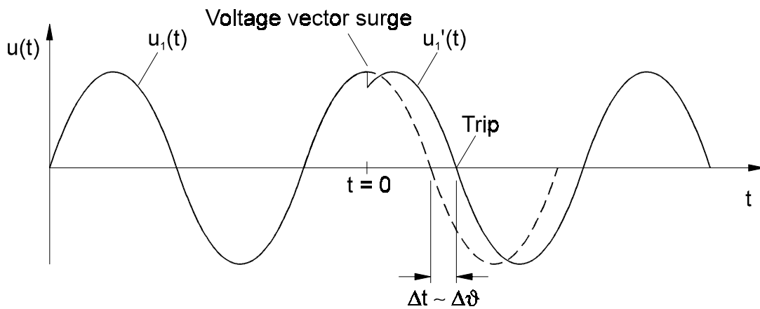
Fig. 3.5: Voltage vector shift
