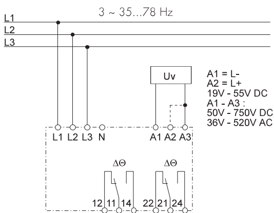
Fig. 2.2: Connection three-wire system \Delta
