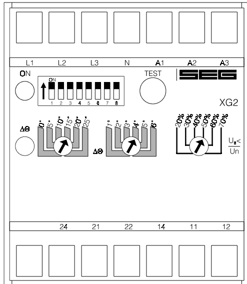
Fig. 4.1: Front plate
