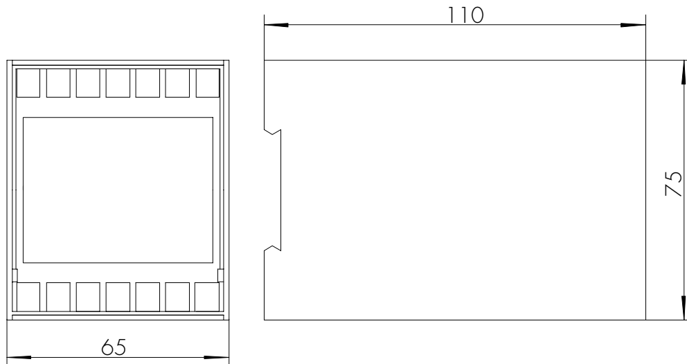
Fig. 5.1: Dimensional drawings
