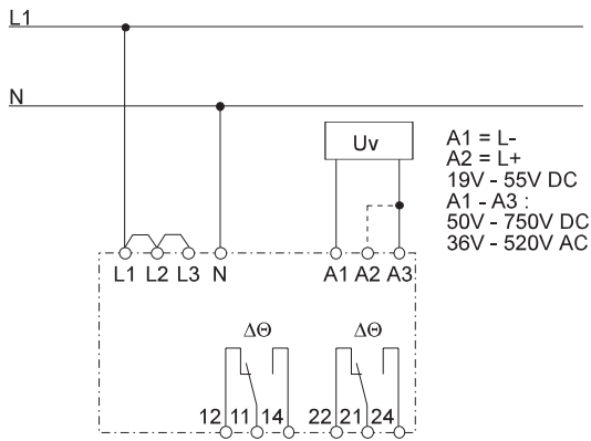
Fig. 2.1: Connection two-wire system
