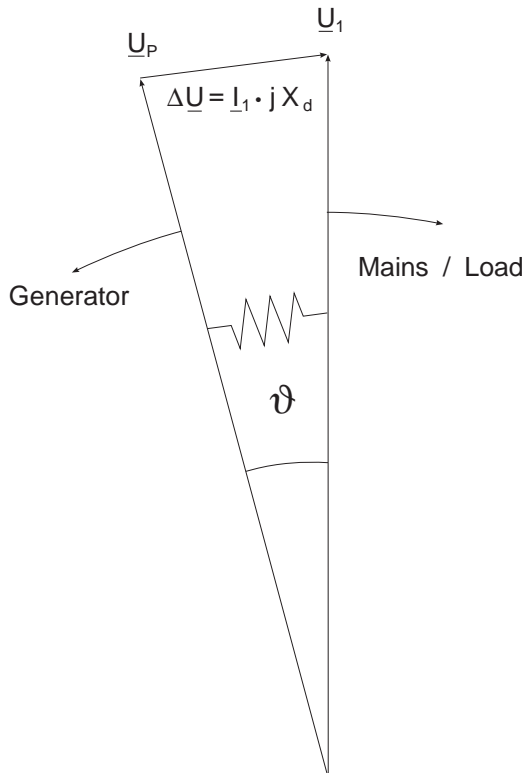
Fig. 3.2: Voltage vectors at mains parallel operation
