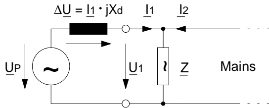
Fig. 3.1: Equivalent circuit of synchronous generator in parallel with the mains
