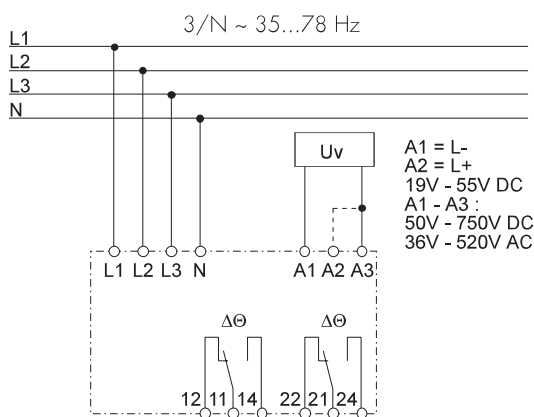
Fig. 2.3: Connection four-wire system Y/ \Delta
