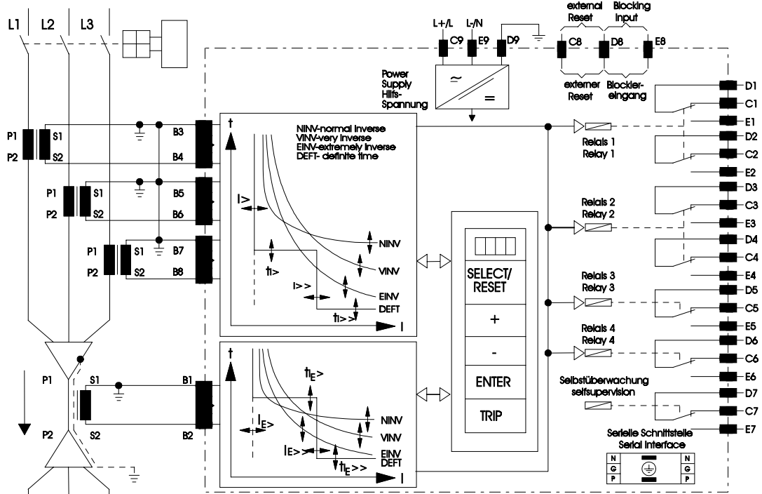
Figure 3.1: Connection diagram
