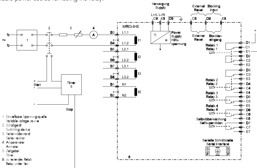
Figure 6.1: Test circuit
