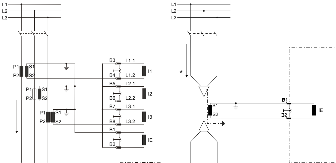
Figure 3.1: Connection diagram
