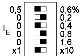
Fig. 6.1: Setting example for the earth fault current pickup value
