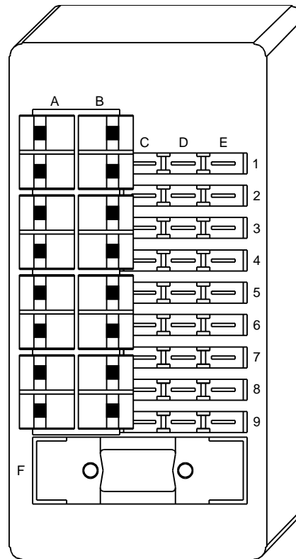
Fig. 7.1: Terminal block
