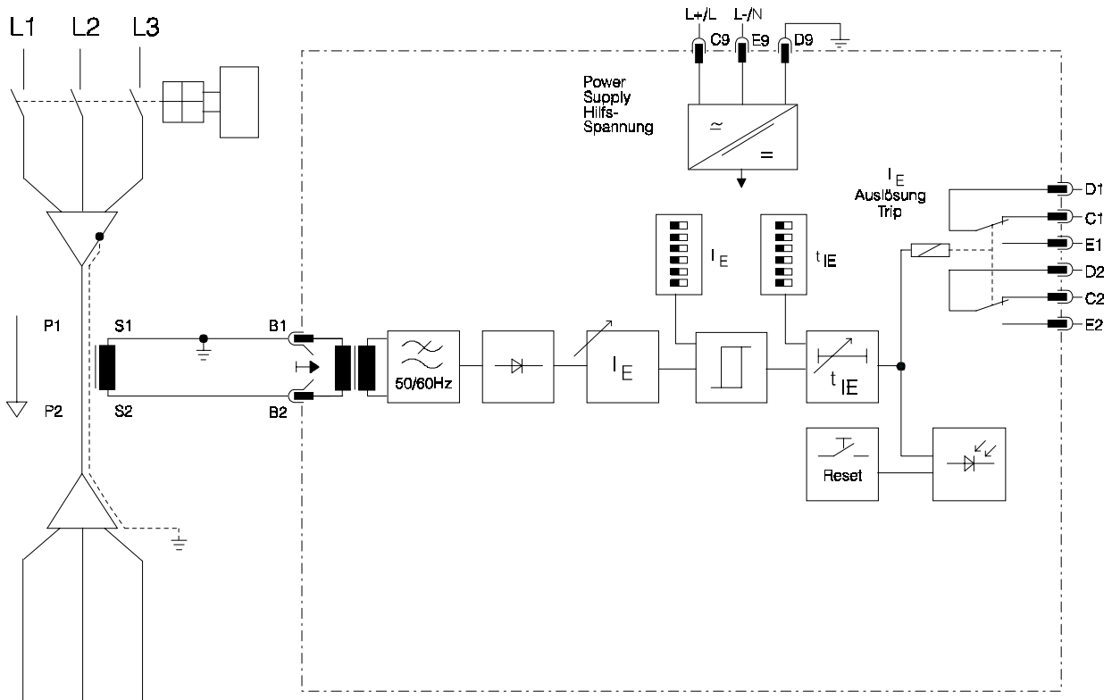
Fig. 4.1: Connection diagram of IRI1-ES
