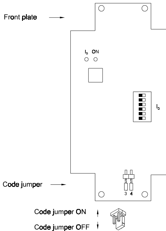
Fig. 4.3: Code jumpers
